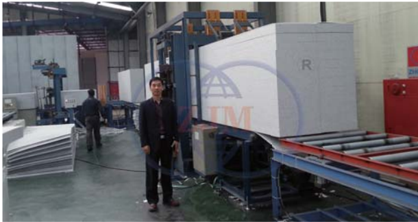
7. 带自动调丝的板材振动切割、打包 Block vibration cutting with automatic adjusting wire system & packaging
